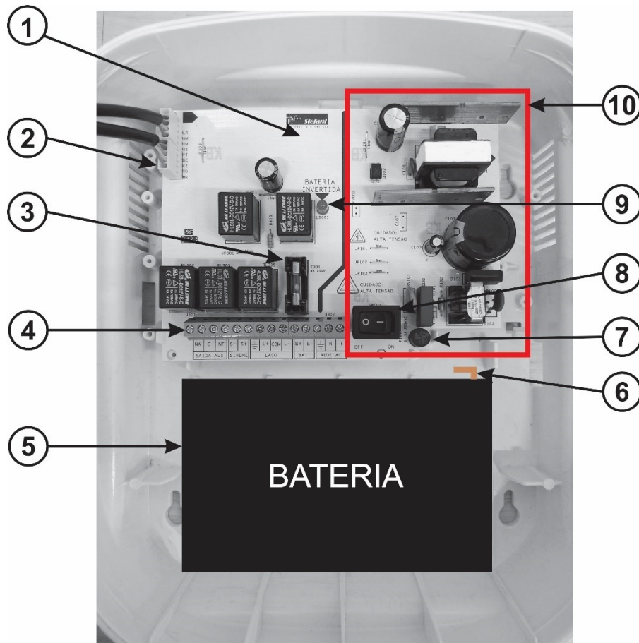
Figura 2. 2: Legenda interna Central
