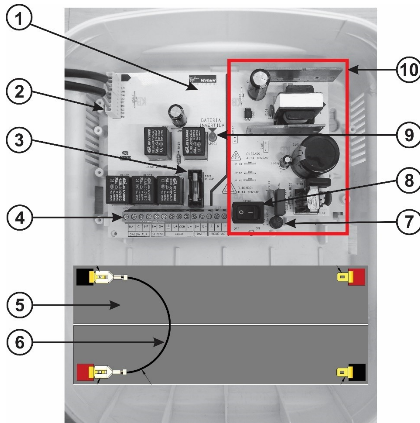
Figura 2. 2: Legenda interna Central
